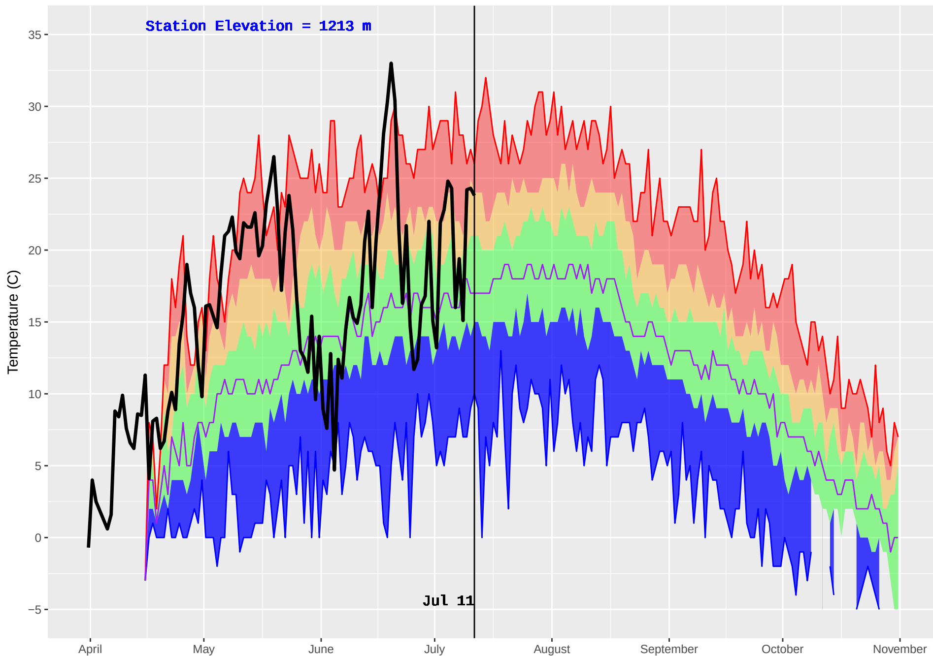
INGENIKA POINT (145) : Historical (1971–2016) and Current (2018) Noon Temperature
