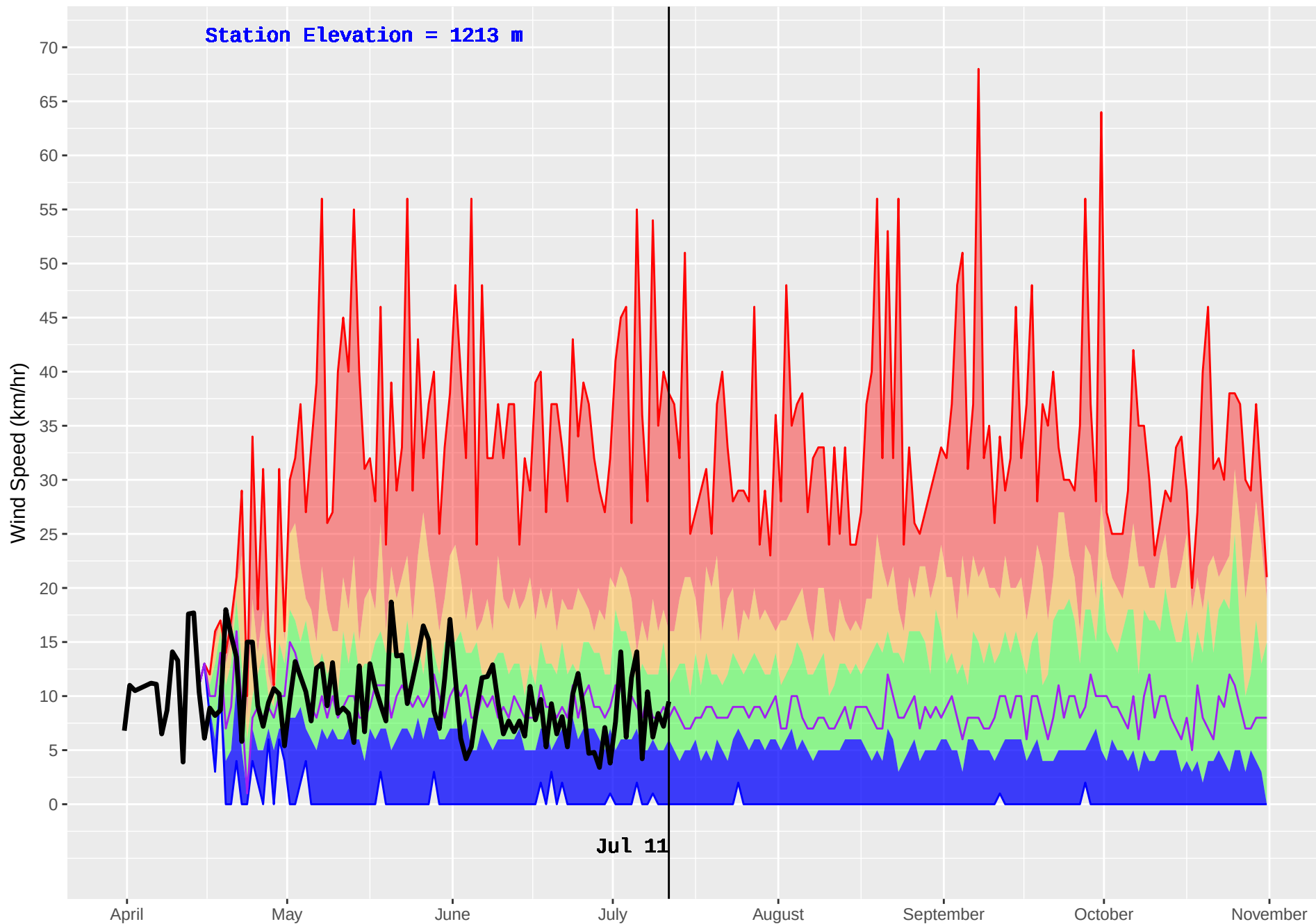
INGENIKA POINT (145) : Historical (1971–2016) and Current (2018) Noon Wind Speed
